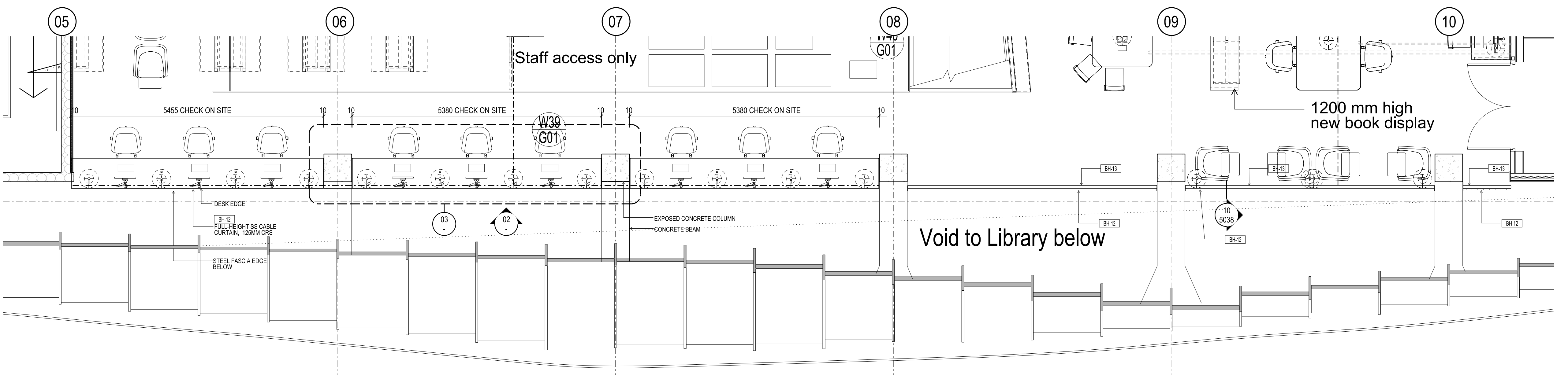
01 PLAN - JOG-05 VOID EDGE DESK / BH-12 SS BALUSTRADE SCALE 1:50
