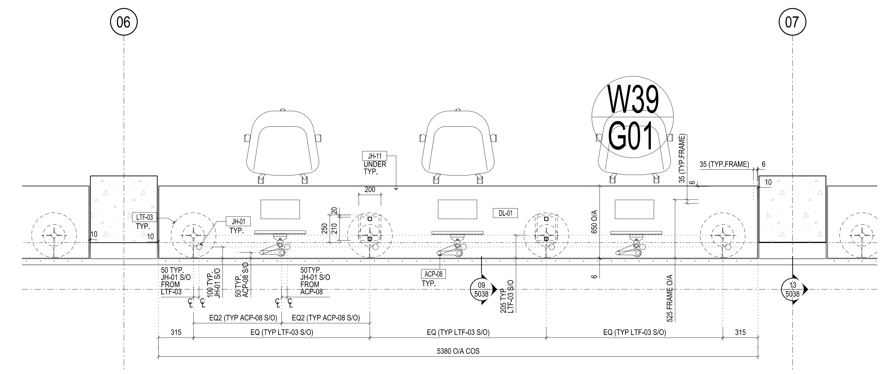
03 PLAN - JOG-05 VOID EDGE DESK / BH-12 SS BALUSTRADE SCALE 1:20
