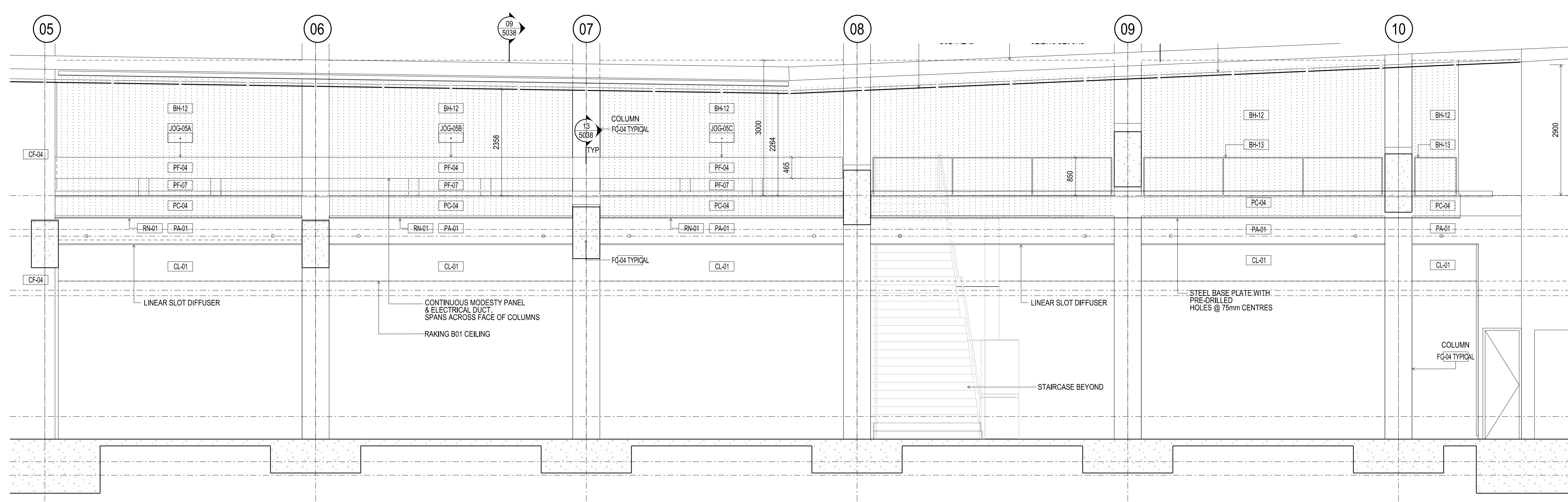
02 ELEVATION - JOG-05 VOID EDGE DESK / BH-12 SS BALUSTRADE SCALE 1:100
